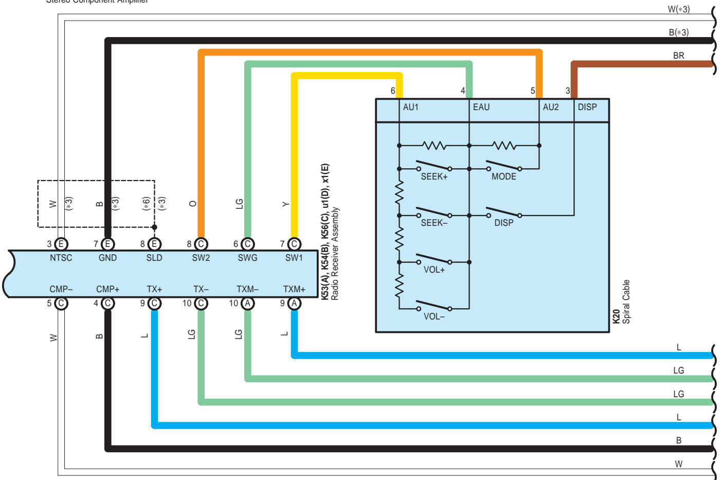
U29(C), U30(D), U31(A), U42(F), U44(G), w1(E) Stereo Component Amplifier
