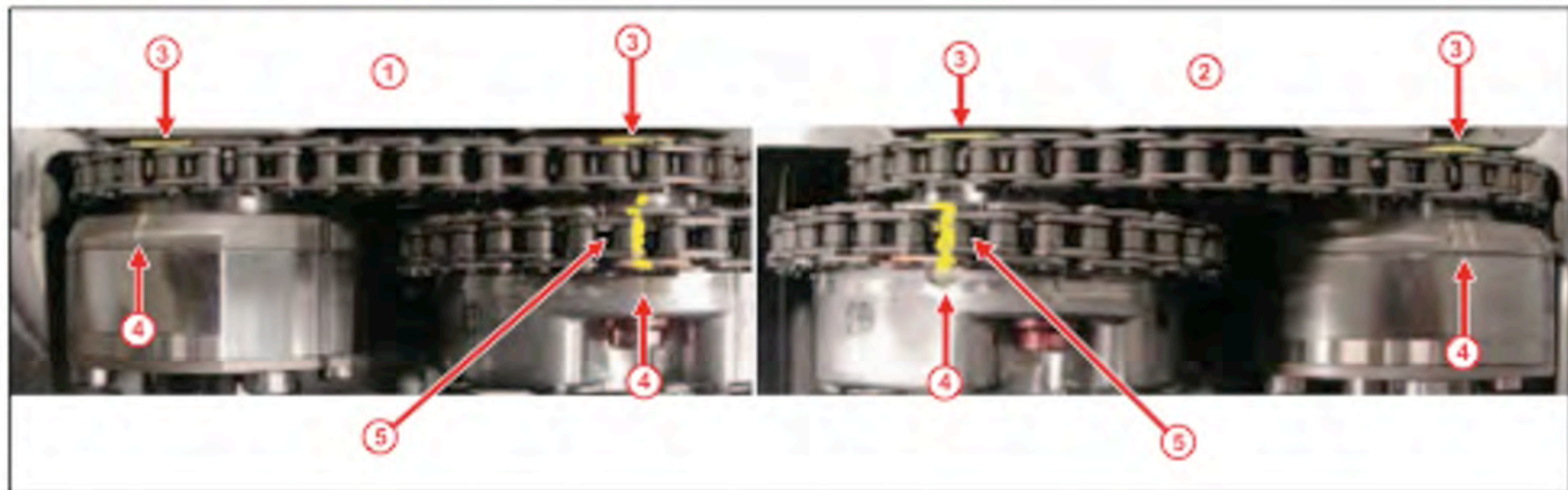
Figure 8. RH Bank and LH Bank
