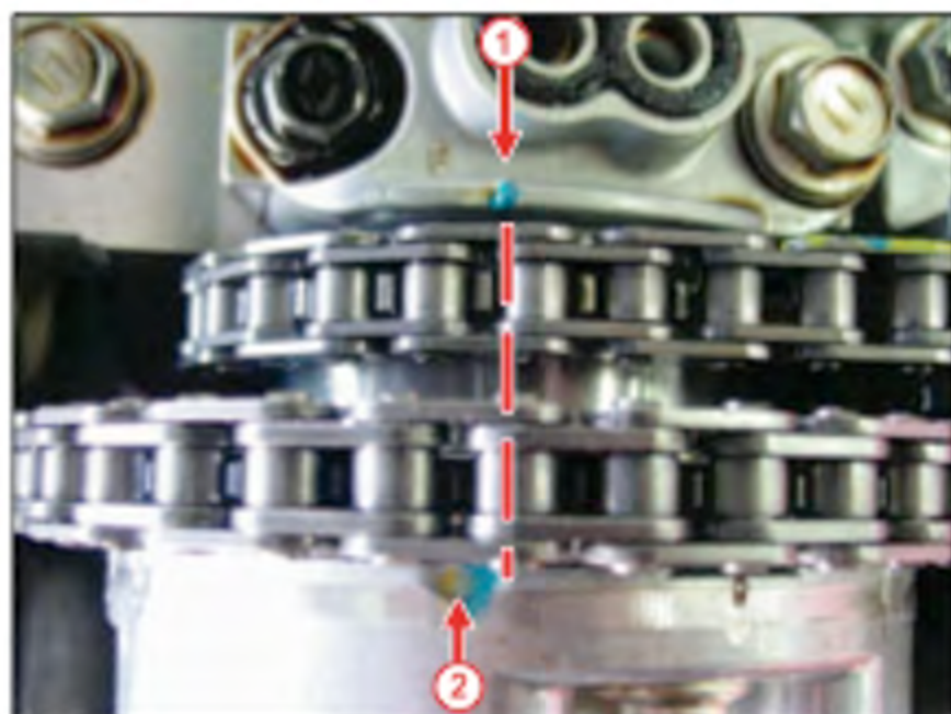
Figure 5. LH Bank Intake Camshaft Timing Gear
