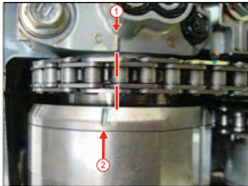
Figure 3. RH Bank Exhaust Camshaft Timing Gear
