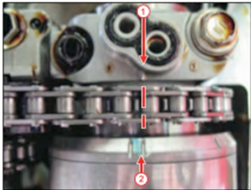
Figure 6. LH Bank Exhaust Camshaft Timing Gear
