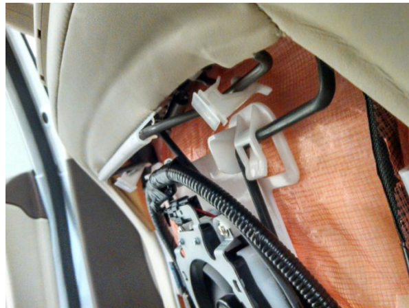
View of the clip once it has been successfully detached from the seatback cover
