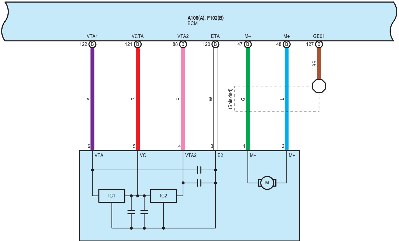
F21 Throttle Body with Motor Assembly
