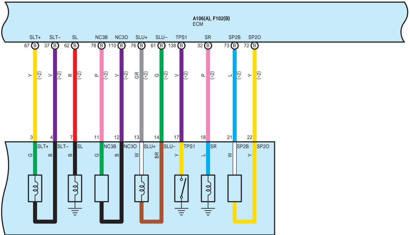
F73 Electronically Controlled Transmission Solenoid (Transmission Wire)
