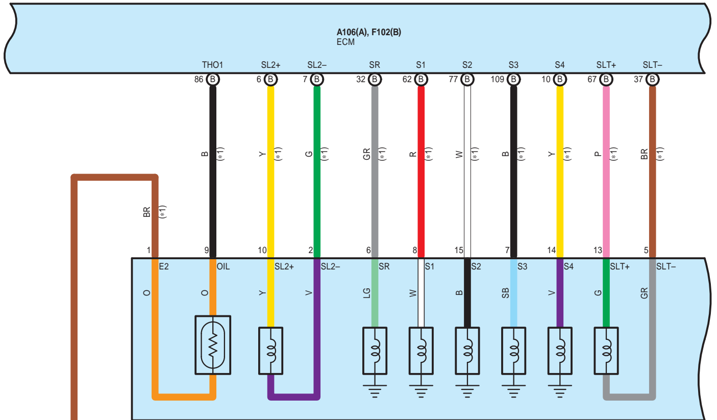
F56 Electronically Controlled Transmission Solenoid (Transmission Wire)
