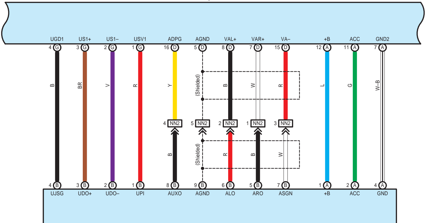
N54(A), N147(B) Stereo Jack Adapter Assembly
