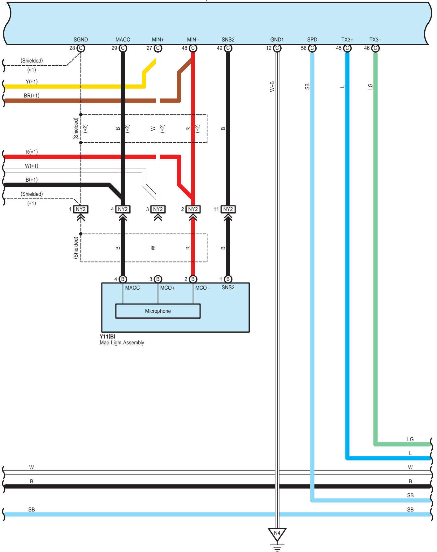
N66(A), N68(C), N69(D), N138(E), N143(J), N146(I), N148(G), N149(H) Multi-Media Module Receiver Assembly
