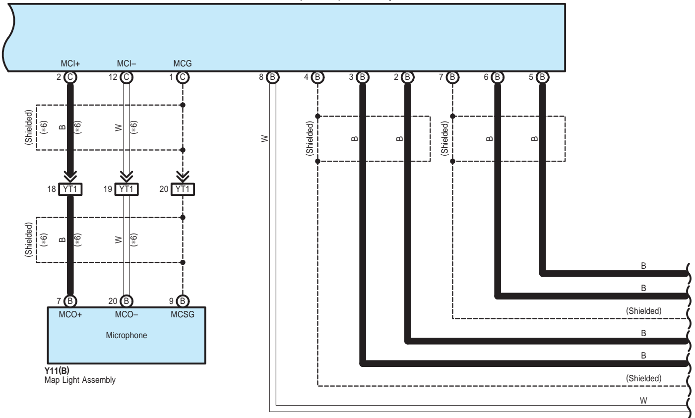
T40(A), T41(C), T49(B) Stereo Component Amplifier Assembly
