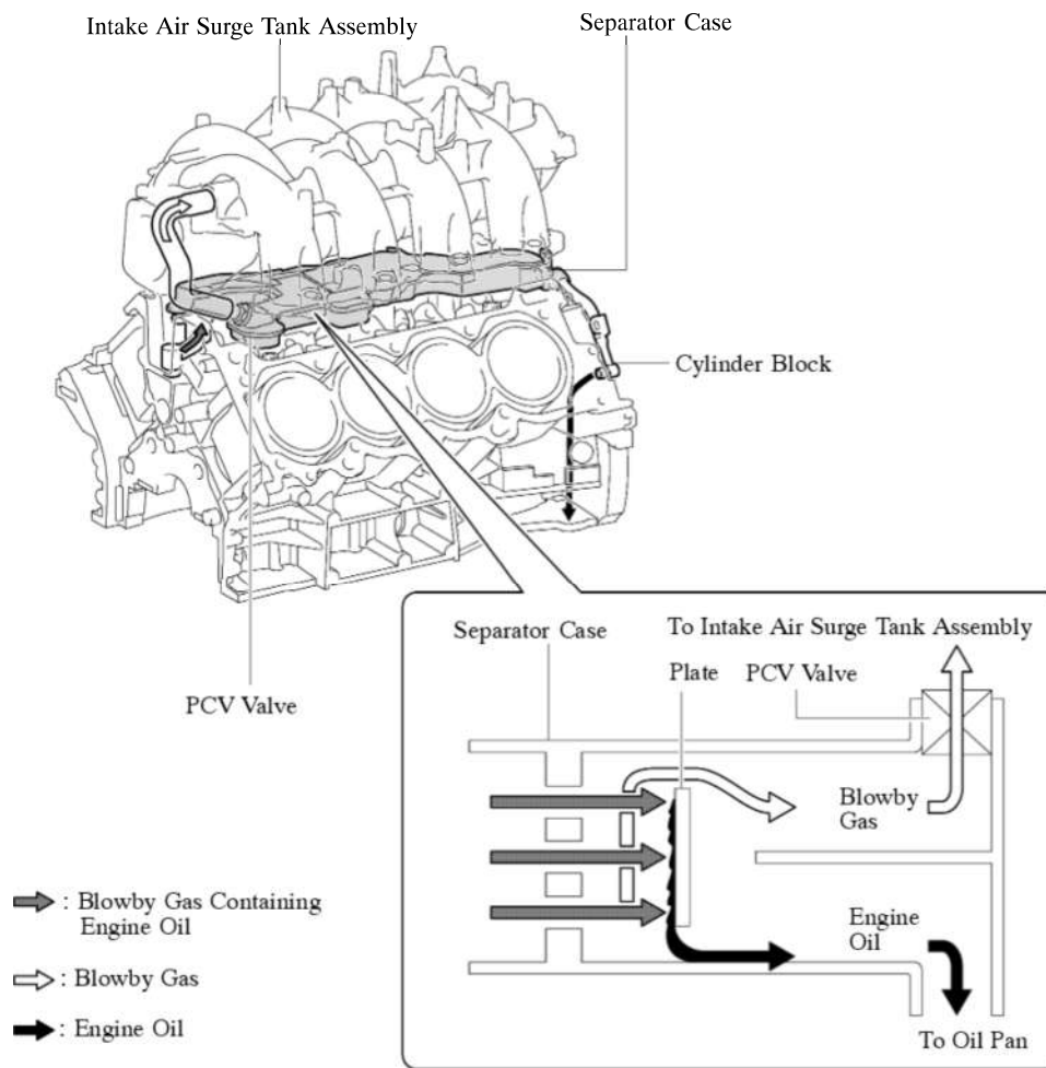
Cross-Sectional Image of Separator Case
