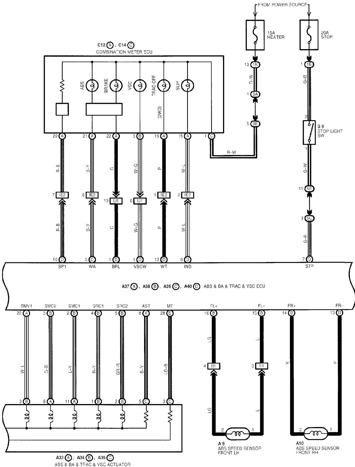
Figure TA2068-10 2001-02 RX300 wiring diagram (sheet 2 of 4)
