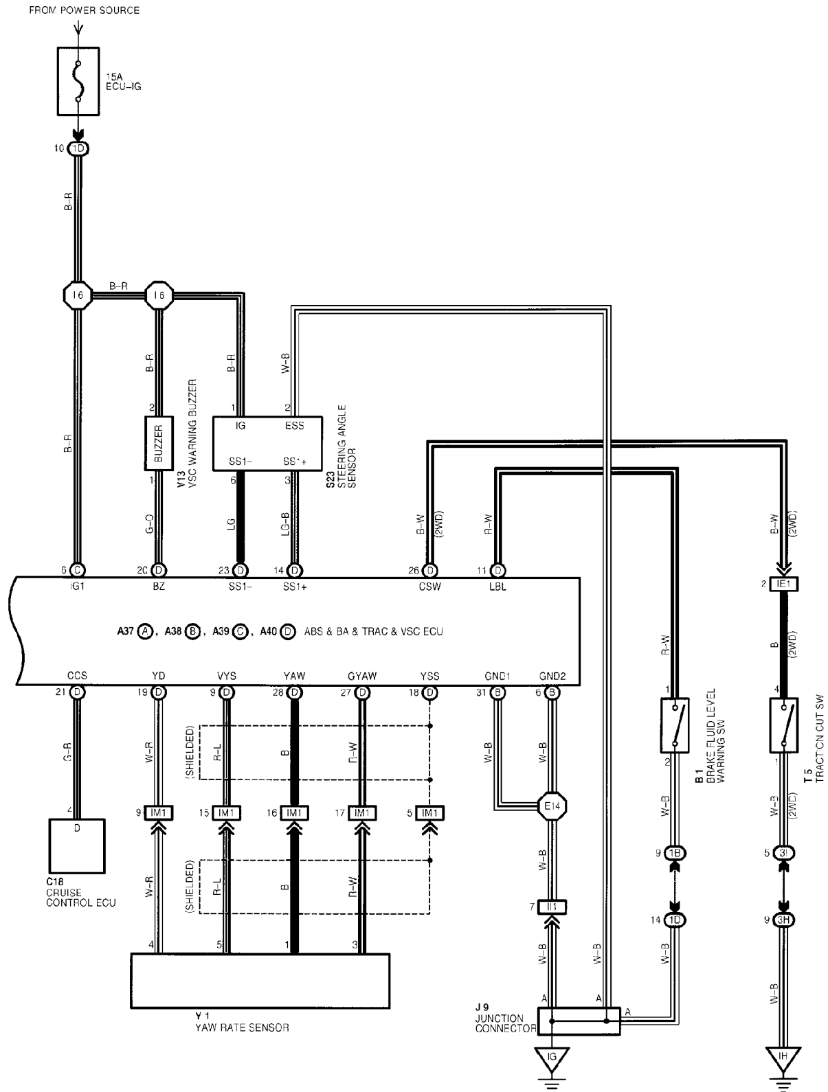
Figure TA2068-10 2001-02 RX300 wiring diagram (sheet 4 of 4)
