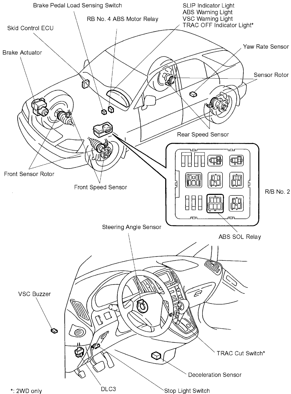
Figure TA2068-12 2003 RX300 component locations
