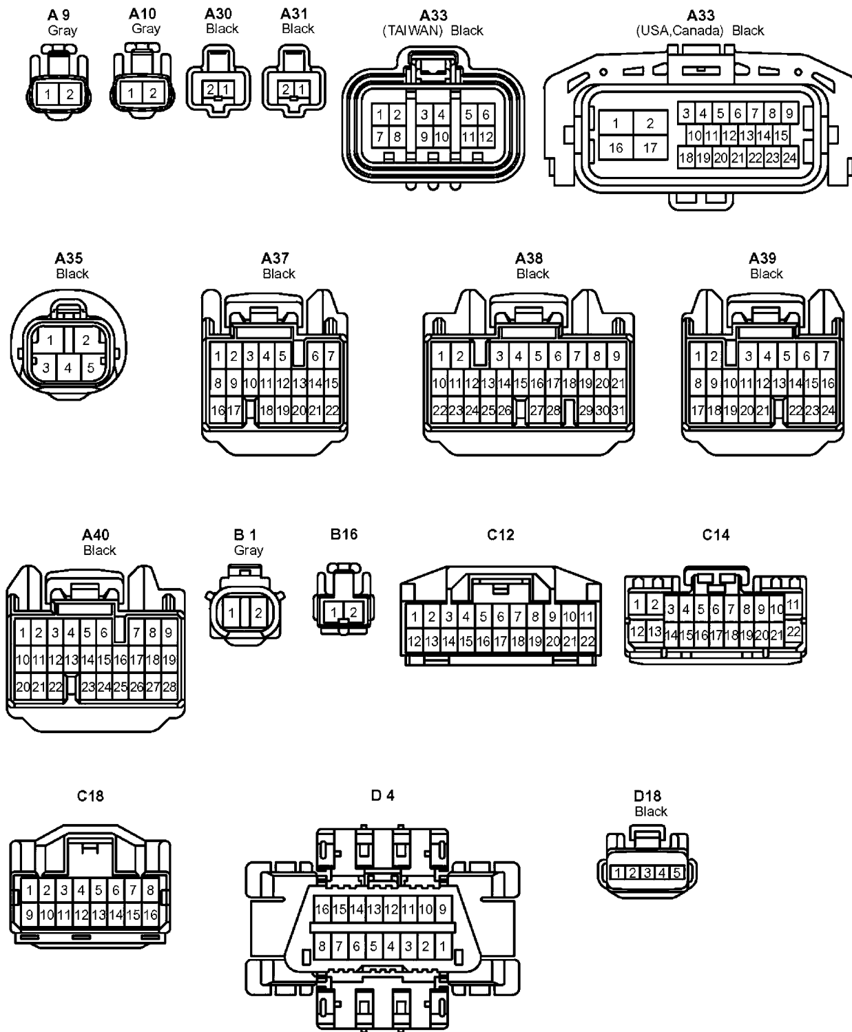
Figure TA2068-14 2003 RX300 connector pinouts (sheet 1 of 2)
