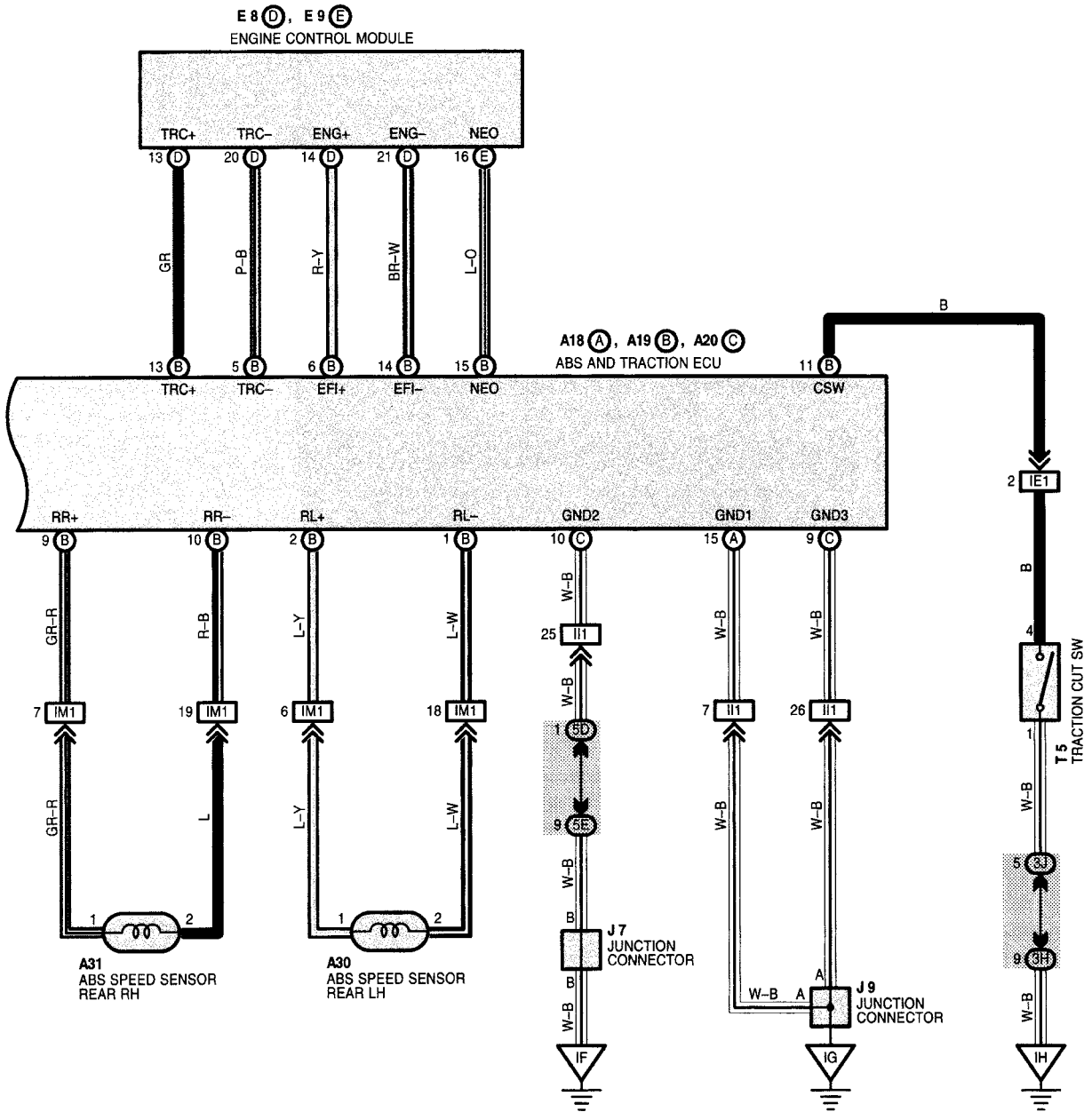
Figure TA2068-4 1999 RX300 (w/TRAC) wiring diagram (sheet 3 of 3)
