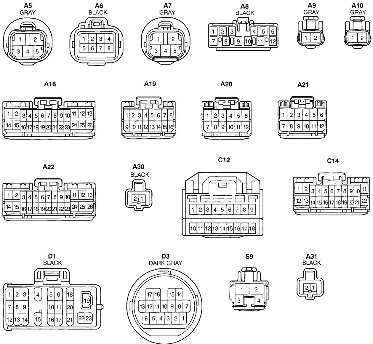
Figure TA2068-5 2000 RX300 connector pinouts
