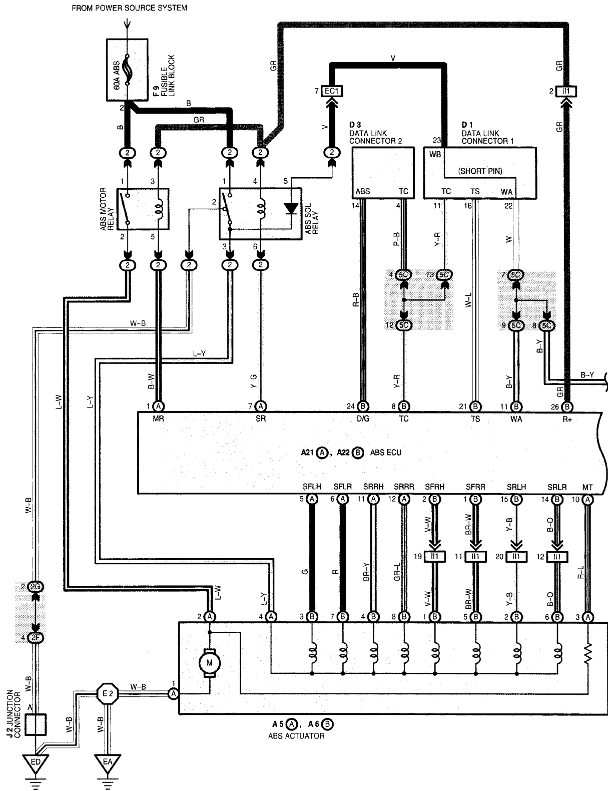
Figure TA2068-3 1999 RX300 (w/o TRAC) wiring diagram (sheet 1 of 2)
