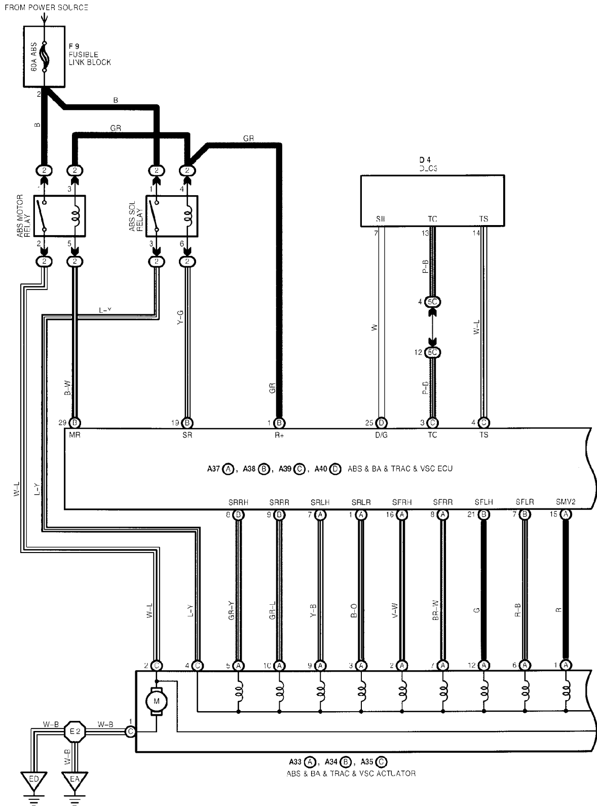
Figure TA2068-10 2001-02 RX300 wiring diagram (sheet 1 of 4)
