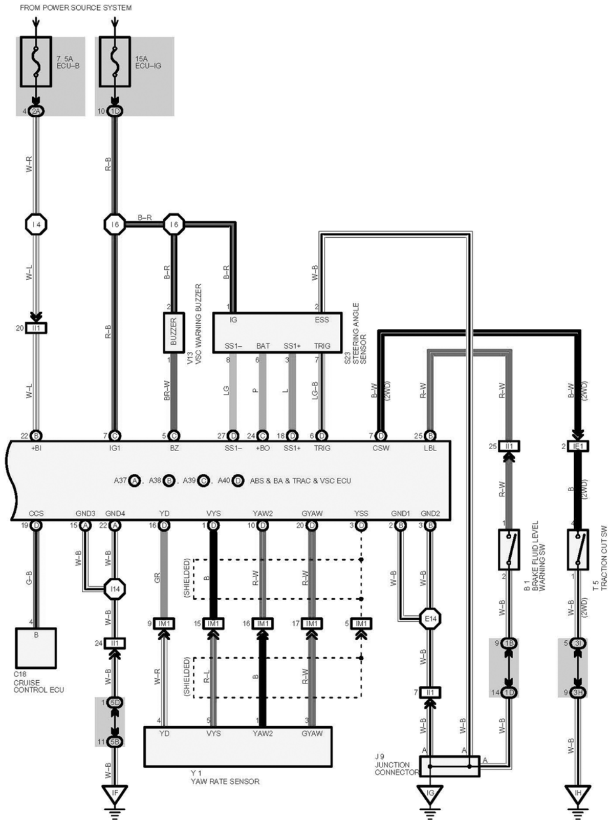
Figure TA2068-13 2003 RX300 wiring diagram (sheet 4 of 4)
