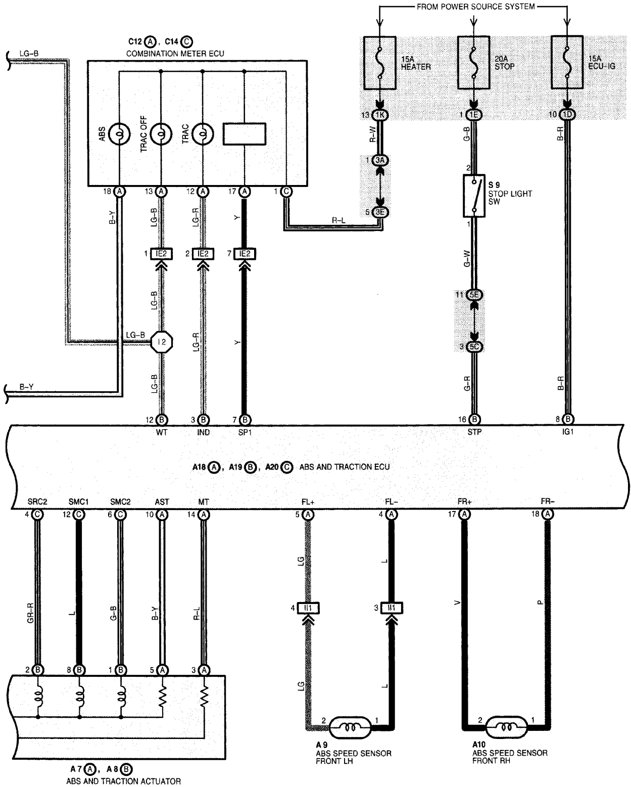
Figure TA2068-4 1999 RX300 (w/TRAC) wiring diagram (sheet 2 of 3)
