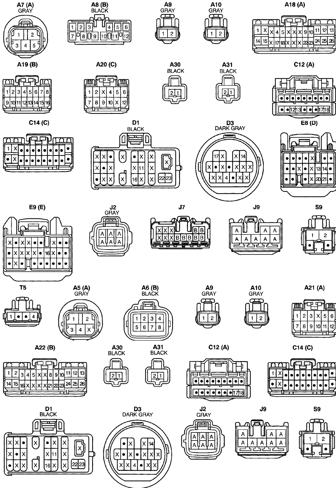
Figure TA2068-2 1999 RX300 connector pinouts
