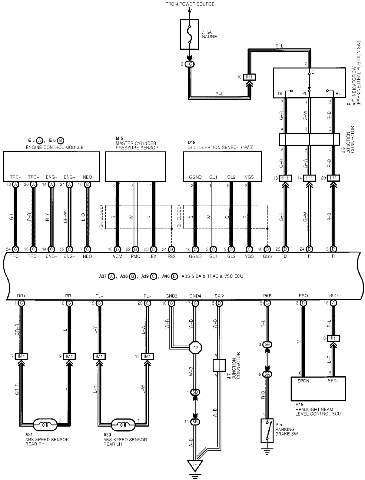
Figure TA2068-10 2001-02 RX300 wiring diagram (sheet 3 of 4)
