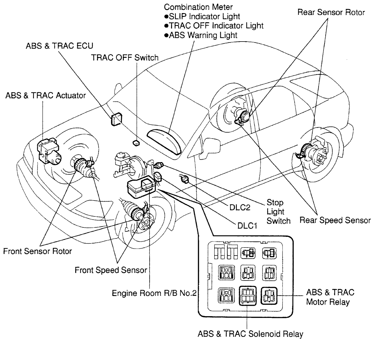
Figure TA2068-1 1999-2000 RX300 component locations
