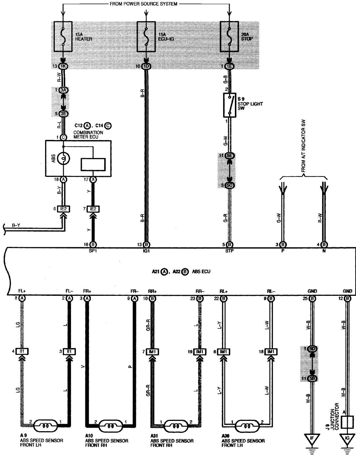
Figure TA2068-3 1999 RX300 (w/o TRAC) wiring diagram (sheet 2 of 2)
