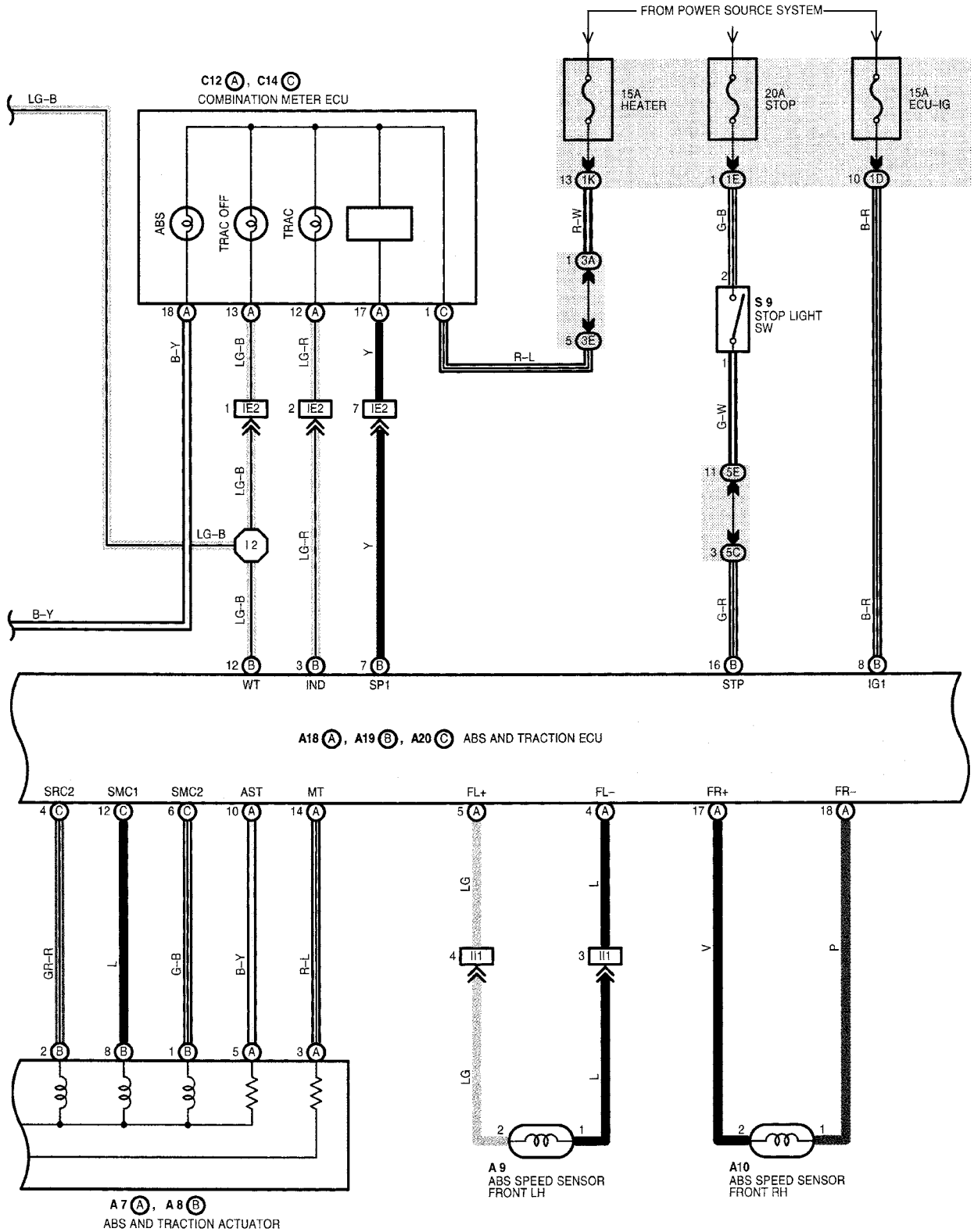
Figure TA2068-7 2000 RX300 (w/TRAC) wiring diagram (sheet 2 of 3)
