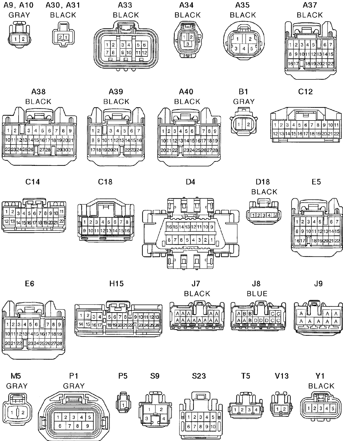
Figure TA2068-9 2001–02 RX300 connector pinouts
