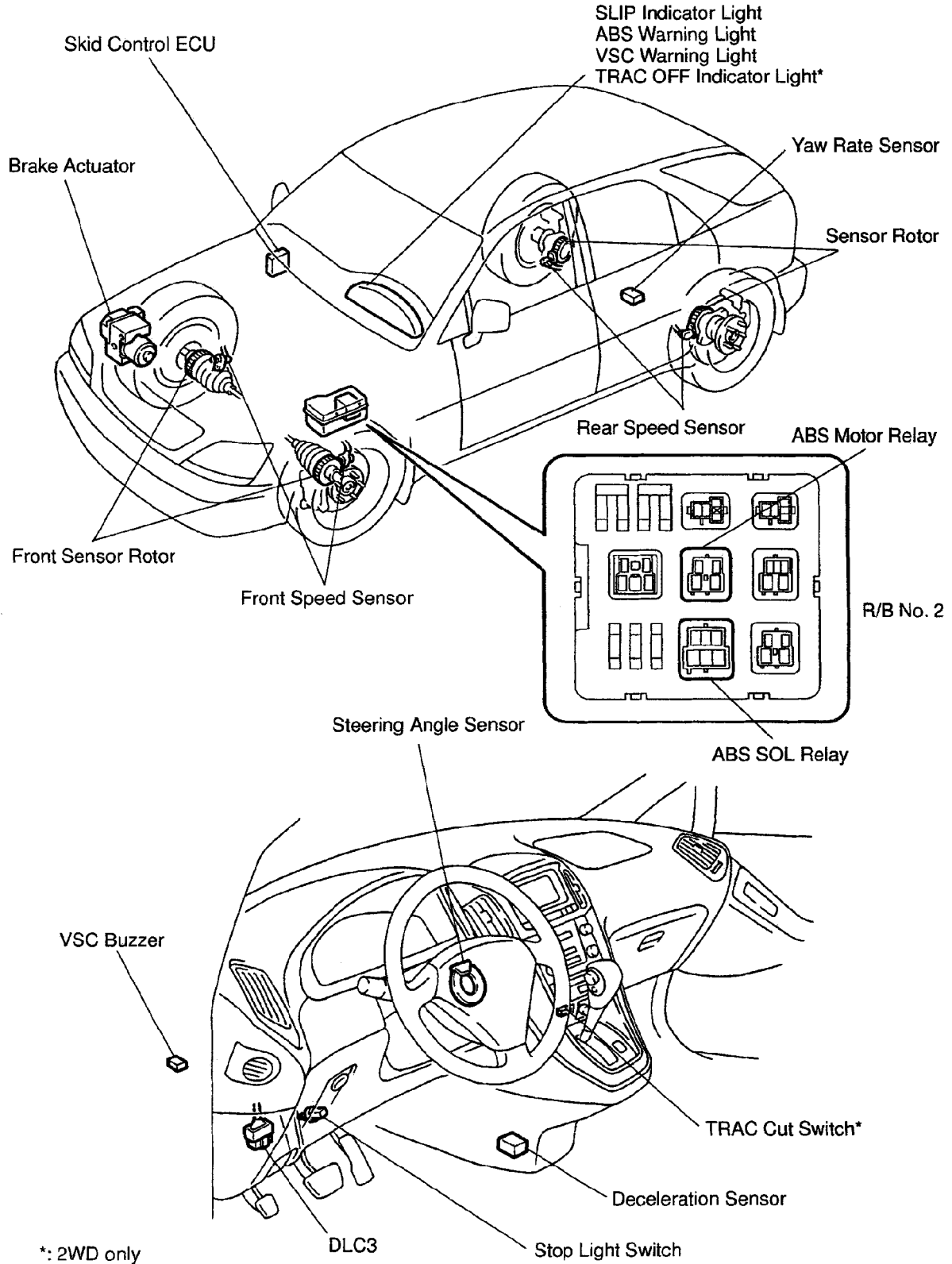
Figure TA2068-8 2001-02 RX300 component locations
