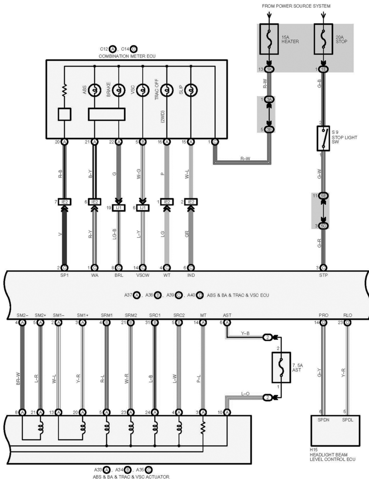
Figure TA2068-13 2003 RX300 wiring diagram (sheet 2 of 4)
