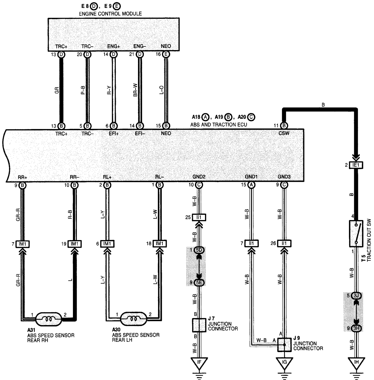
Figure TA2068-7 2000 RX300 (w/TRAC) wiring diagram (sheet 3 of 3)
