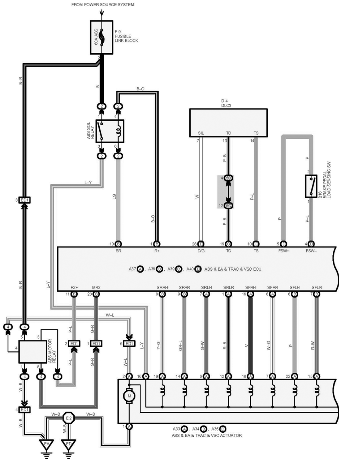
Figure TA2068-13 2003 RX300 wiring diagram (sheet 1 of 4)
