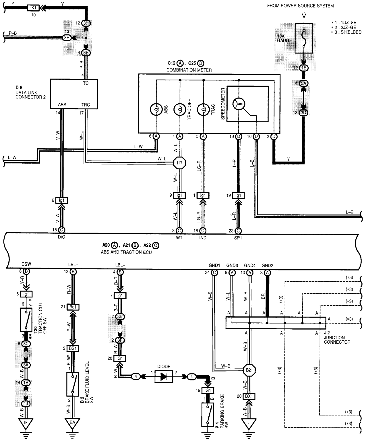
Figure TA2068-6 2000 RX300 (w/o TRAC) wiring diagram (sheet 1 of 2)
