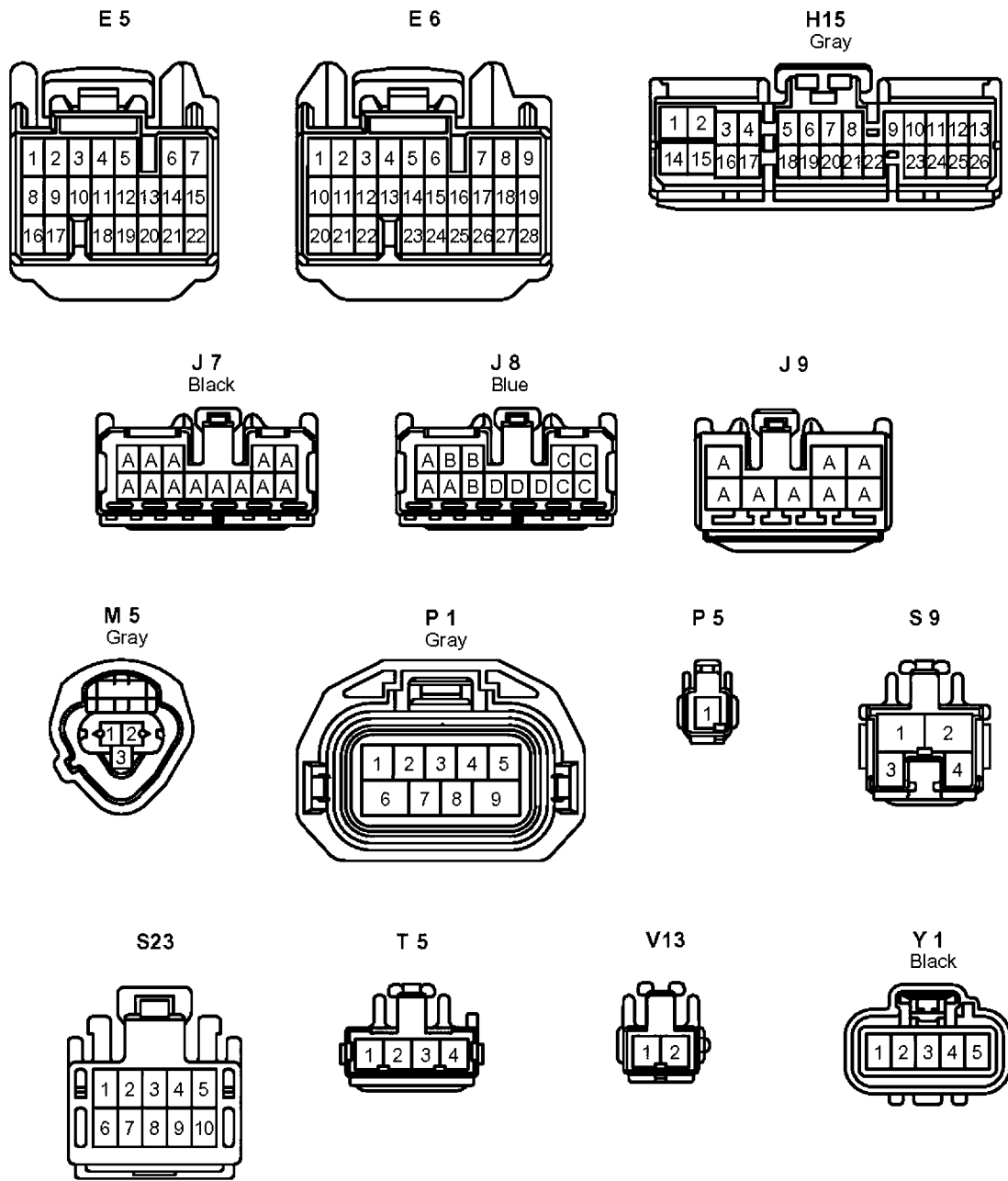
Figure TA2068-14 2003 RX300 connector pinouts (sheet 2 of 2)
