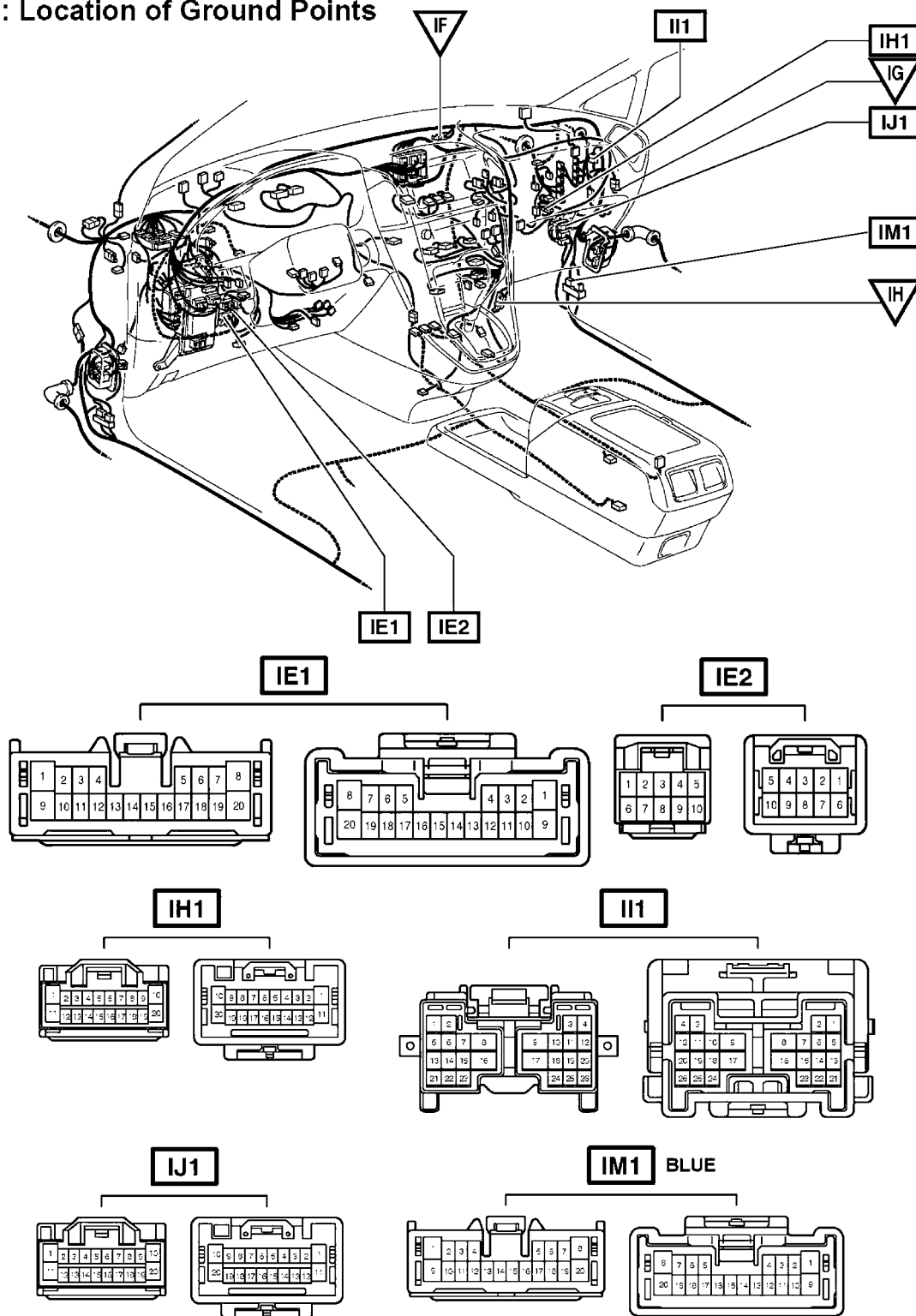
Figure TA2068-11 2001 - 2003 RX300 connector joints and grounds (sheet 2 of 2)
