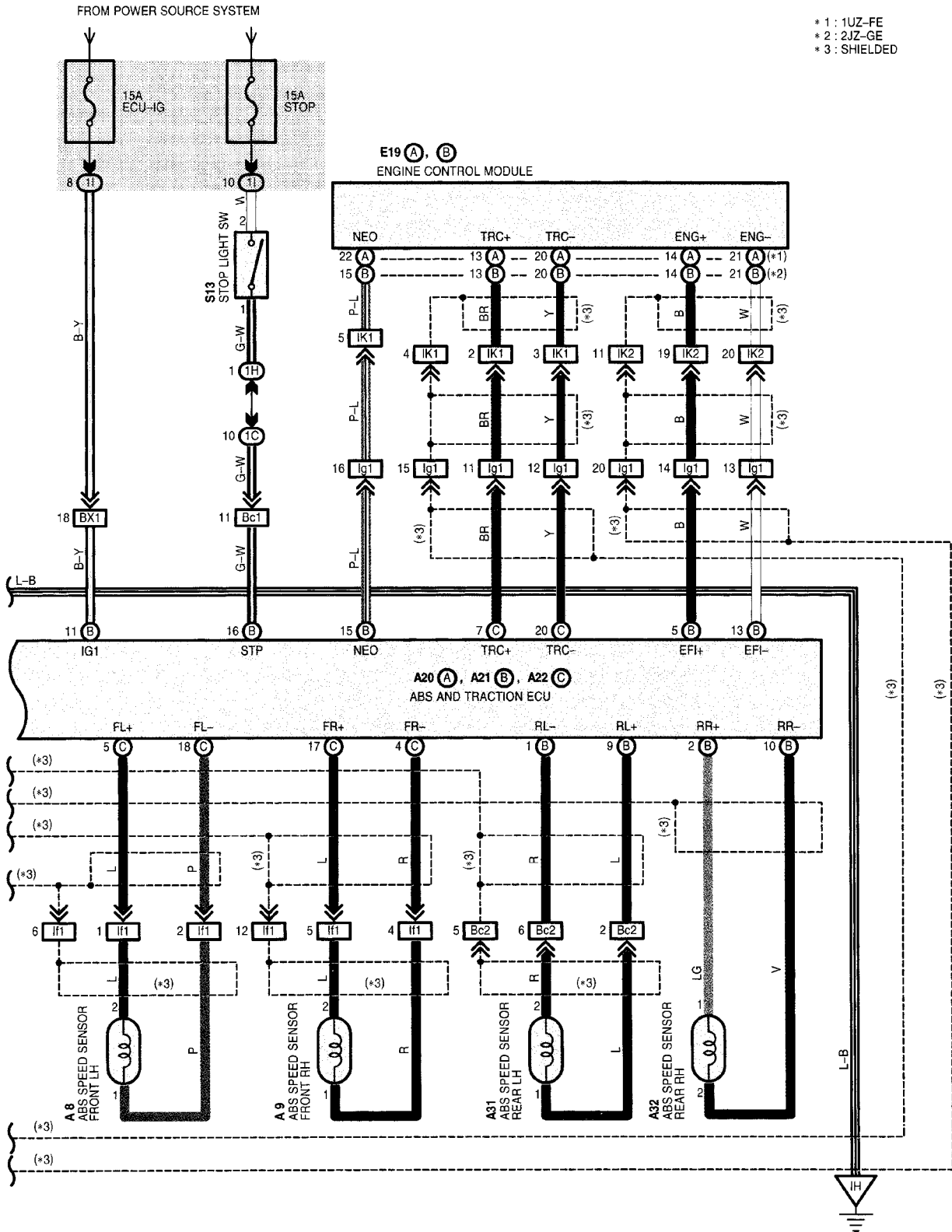
Figure TA2068-6 2000 RX300 (w/o TRAC) wiring diagram (sheet 2 of 2)
