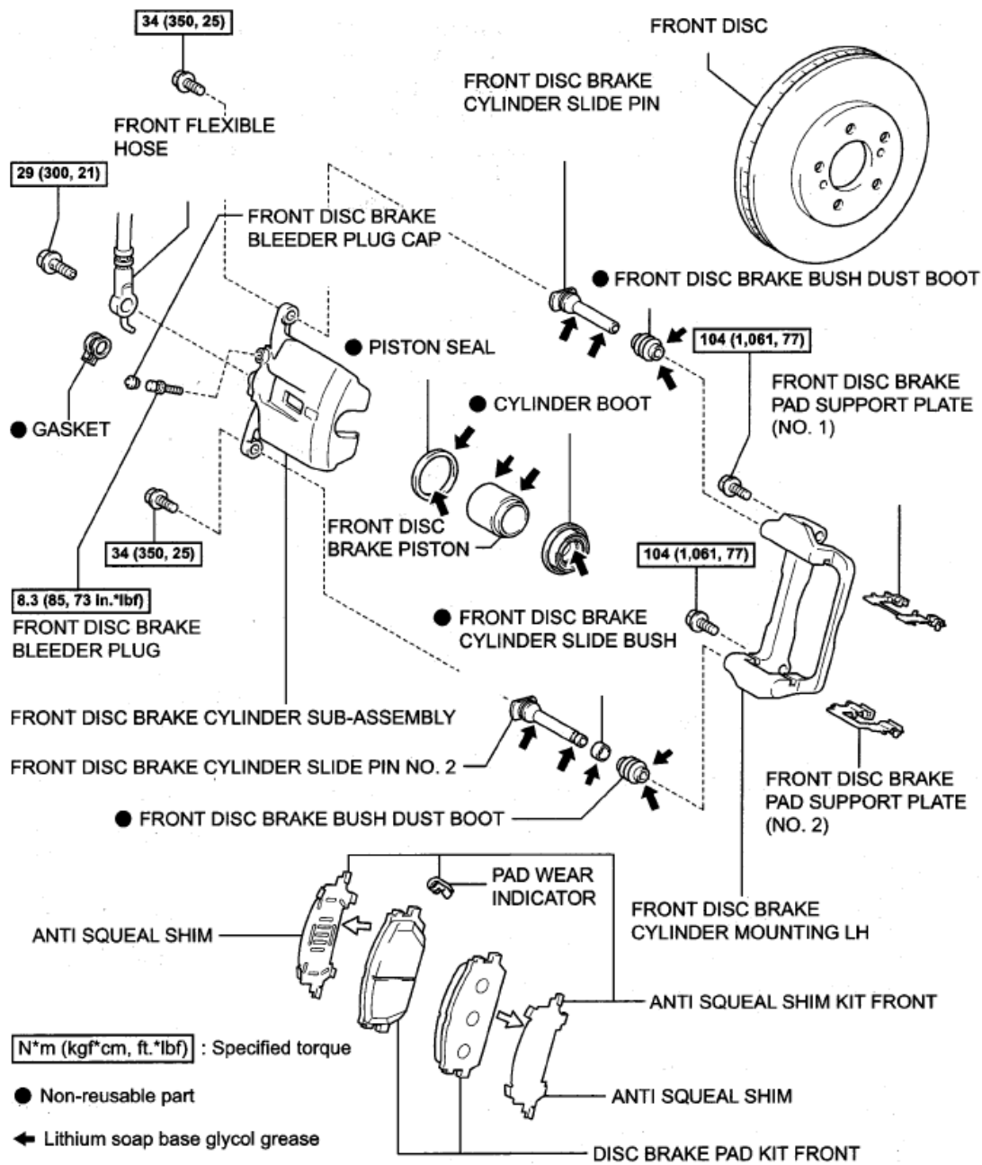
Fig. 42: Identifying Front Brake Replacement Components With Torque Specifications Courtesy of TOYOTA MOTOR SALES, U.S.A., INC.
