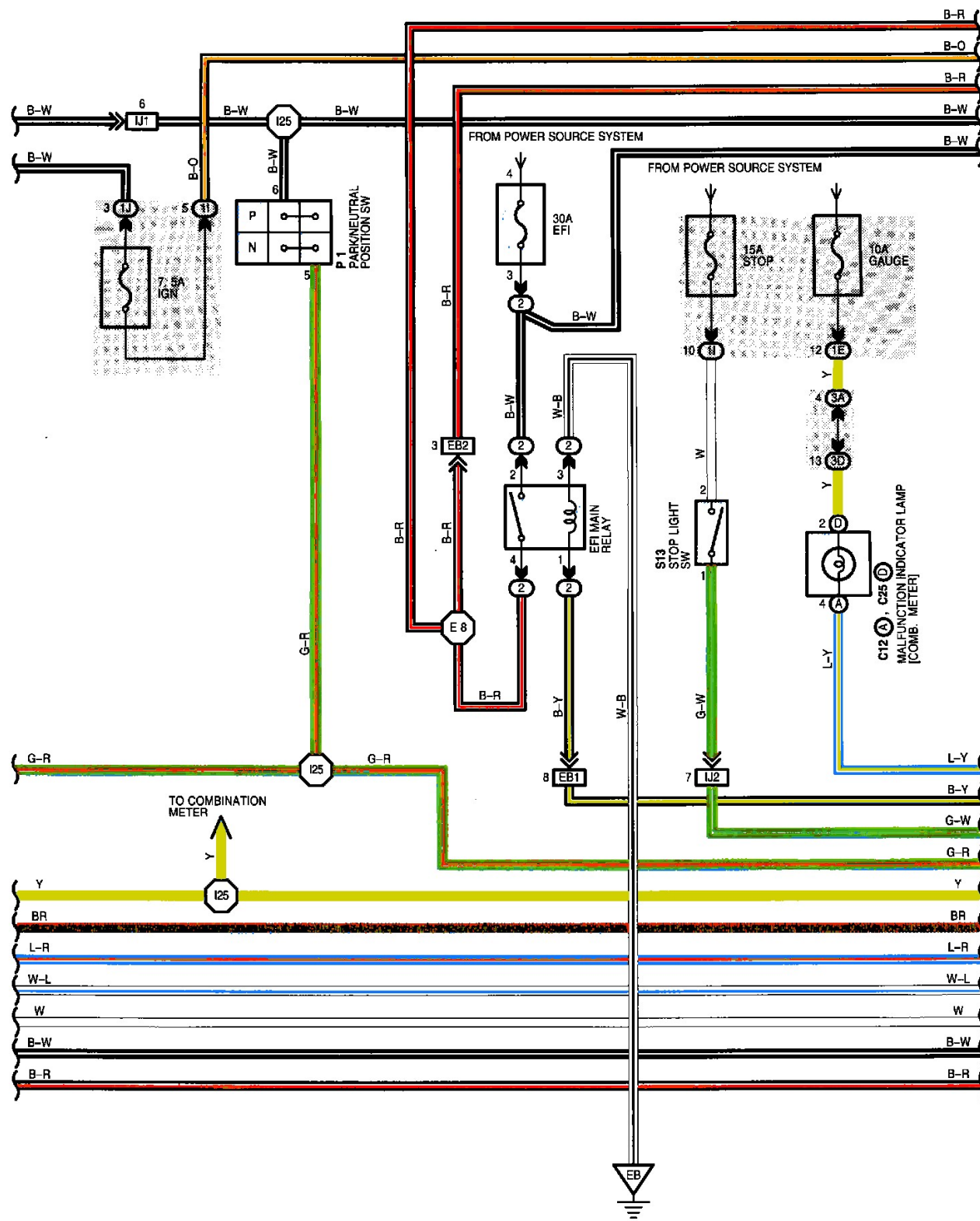
Engine Control And Engine Immobiliser System (Part 2 Of 6)
