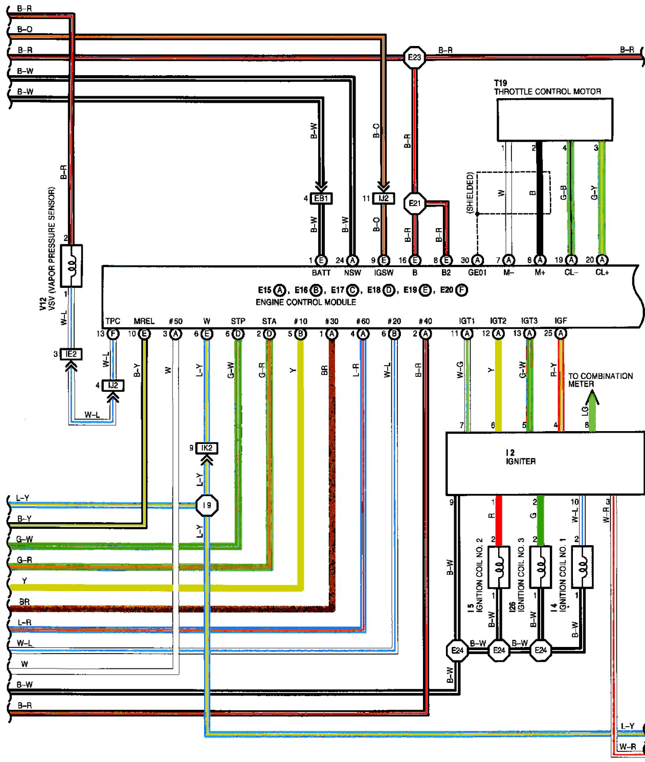
Engine Control And Engine Immobiliser System (Part 3 Of 6)
