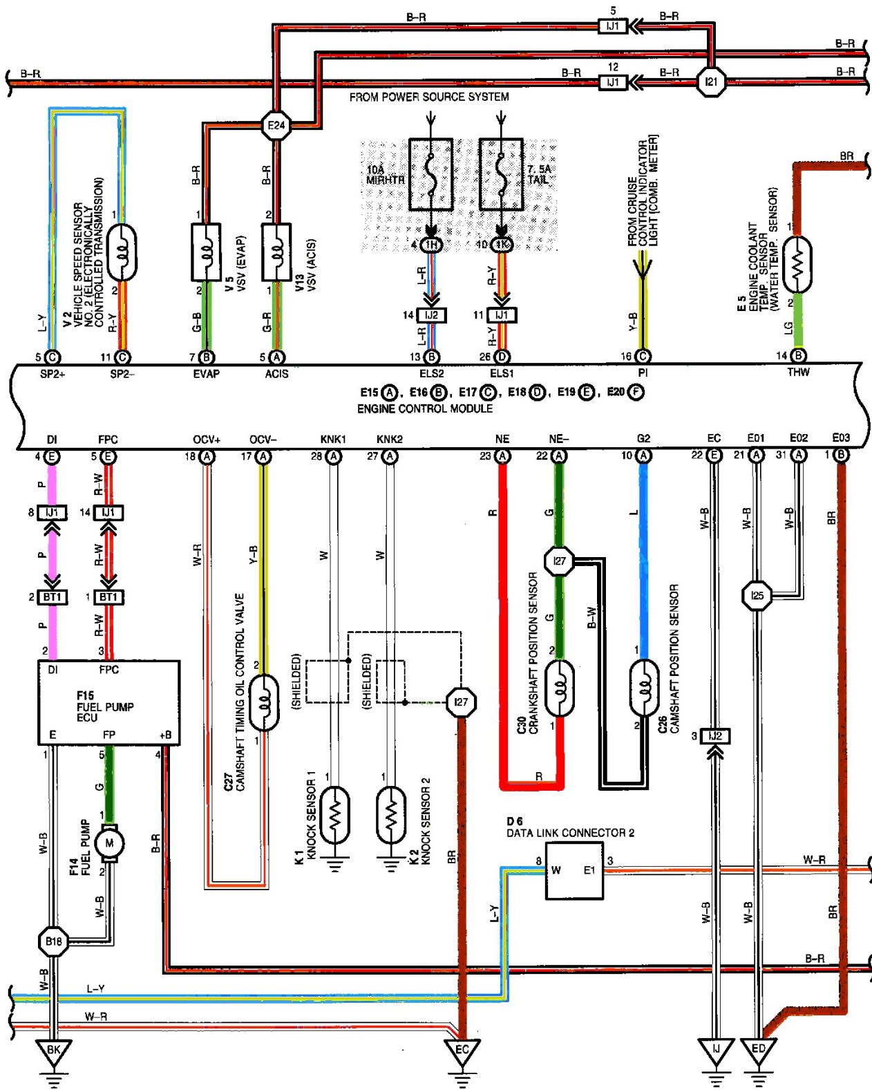
Engine Control And Engine Immobiliser System (Part 4 Of 6)
