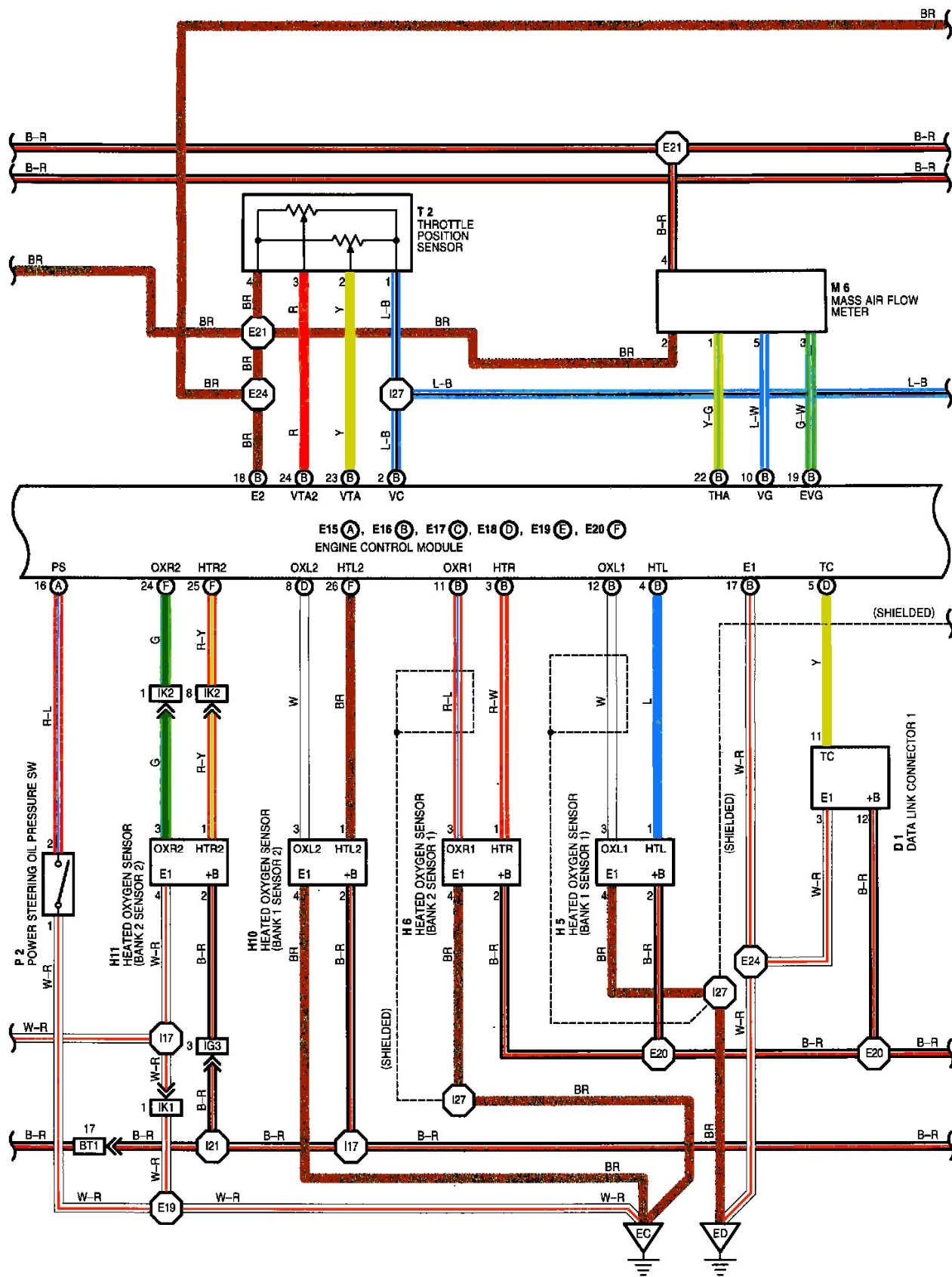
Engine Control And Engine Immobiliser System (Part 5 Of 6)
