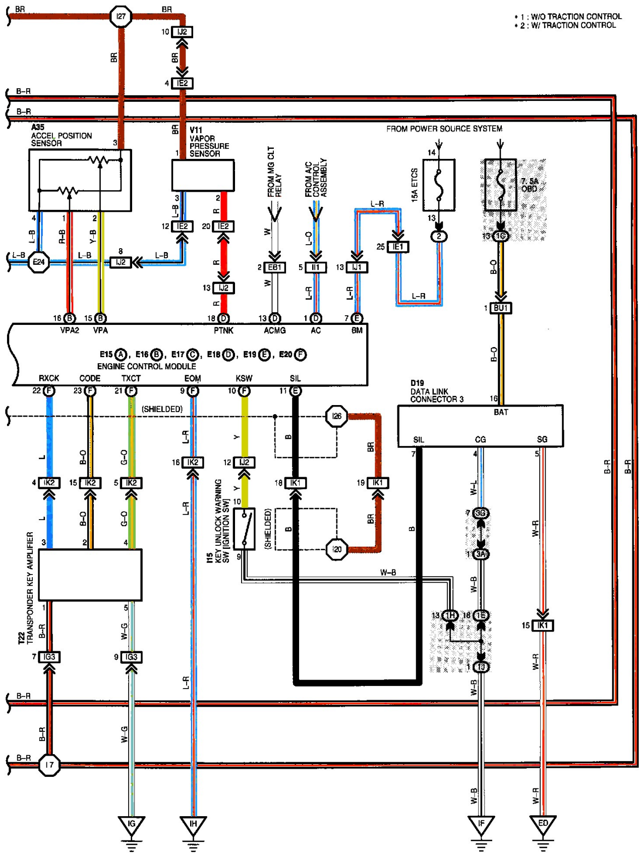
Engine Control And Engine Immobiliser System (Part 6 Of 6)
