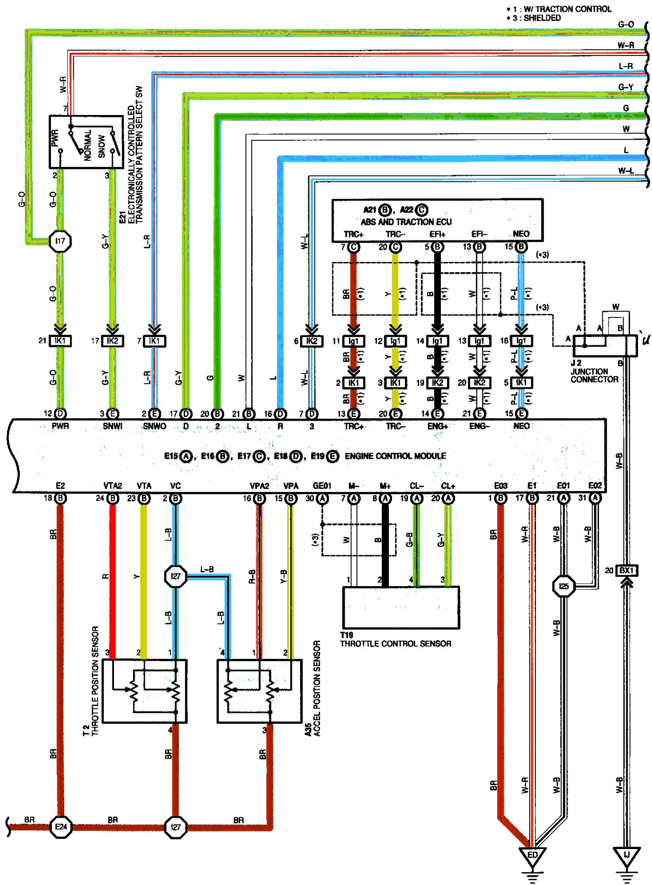
Electronically Controlled Transmission And A/T Indicator (Part 2 Of 3)
