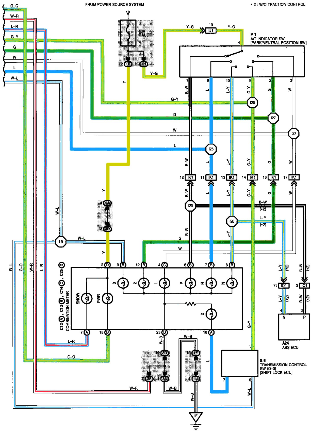
Electronically Controlled Transmission And A/T Indicator (Part 3 Of 3)
