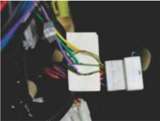
IC1 - 24 pin connector behind L/H carpet kick panel
